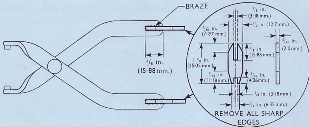
Fig. 1. Modified Loom Pliers for Moulded Type Terminals
